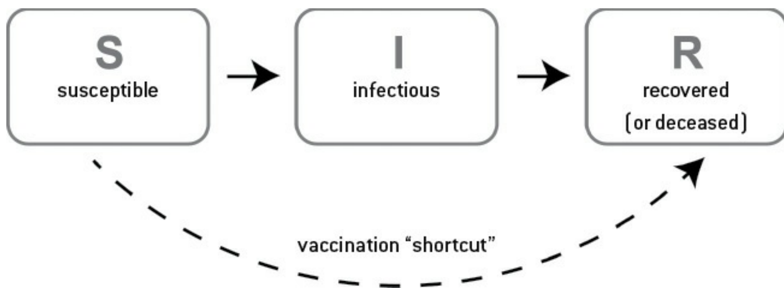
FIGURE 7-5: SCHEMATIC OF SIR MODEL
