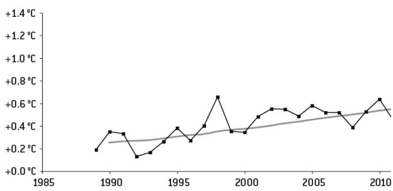
FIGURE 12-9: ACTUAL GLOBAL TEMPERATURES. 1990–2011 VS. SIMPLE REGRESSION FORECAST Anomaly vs. 1951–1980 Baseline
