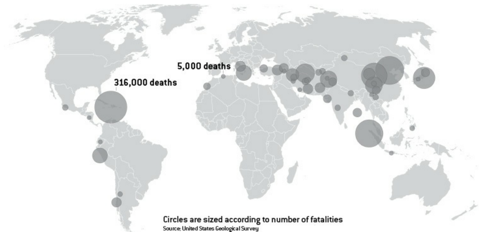
FIGURE 5-1: DEADLIEST EARTHQUAKES SINCE 1900
