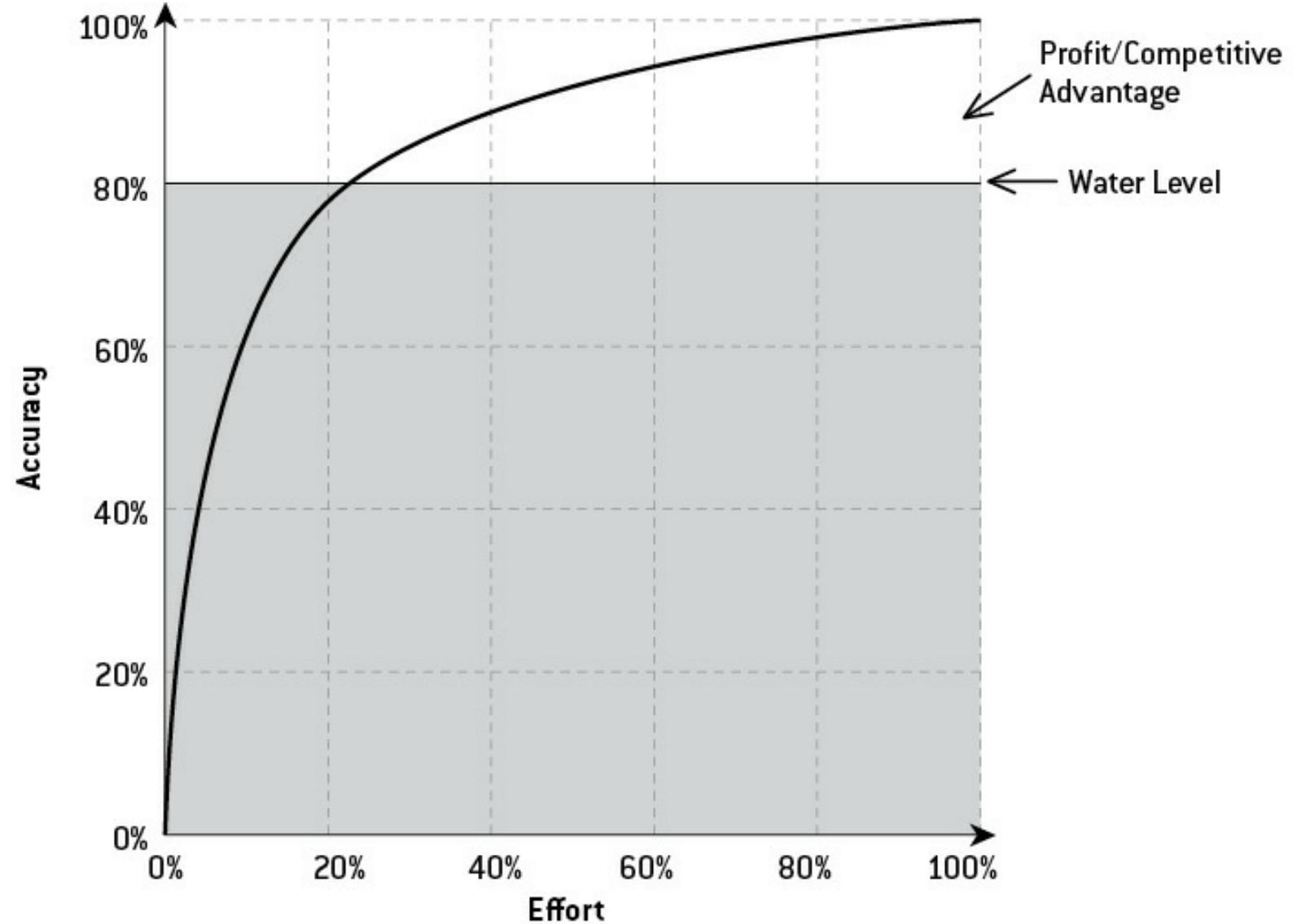
FIGURE 10-7: THE PARETO PRINCIPLE OF PREDICTION IN COMPETITIVE ENVIRONMENTS
